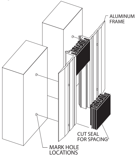
Fig. 1 (104-A07 Wall to Wall shown)
