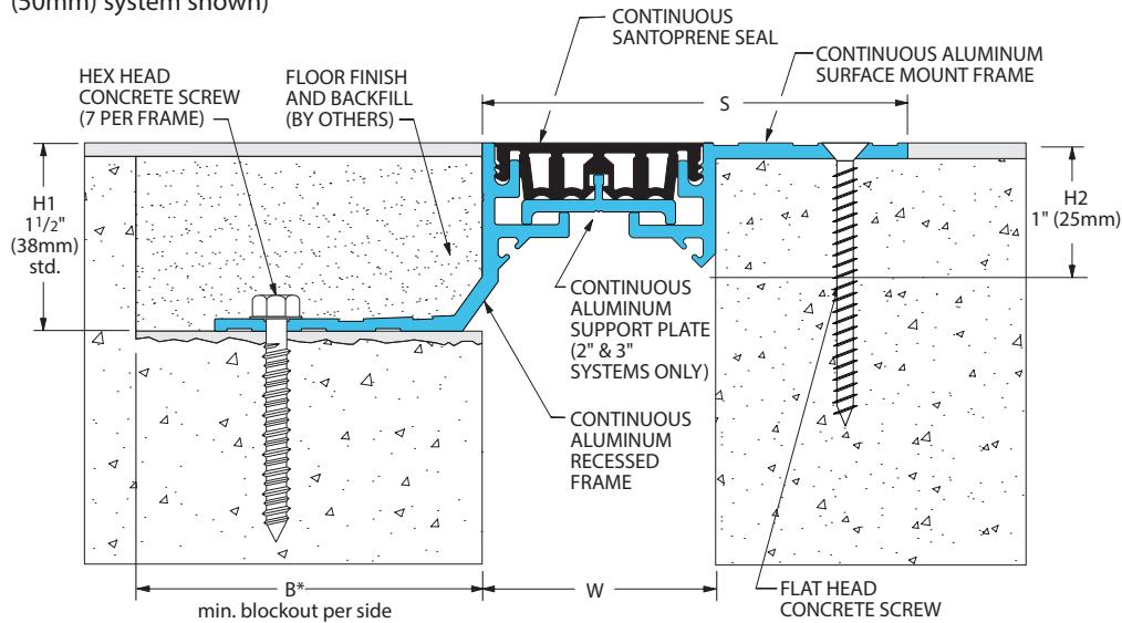
110-A01 Floor/Floor for VCT (2" (50mm) system shown)
