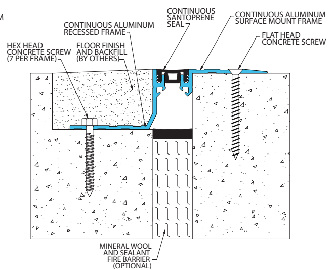
Fire Barrier (107-A01-025 system shown)
