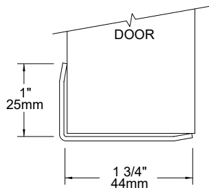
SAS-190CMT ADHESIVE MOUNT TYPE 430, 16 GAUGE
