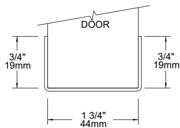
SAS-290CMT SAS-290HOLE-P ADHESIVE & SCREW-ON TYPE 430, 16 GAUGE
